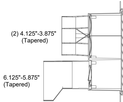
SECTIONAL VIEWS
