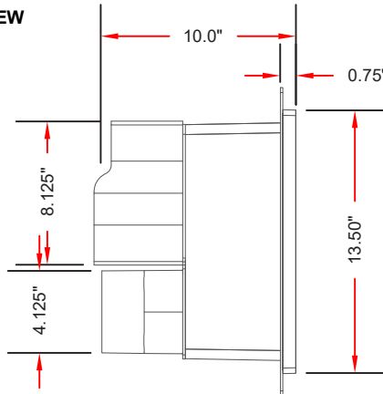
SECTIONAL VIEWS
