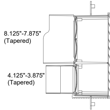
SECTIONAL VIEWS
