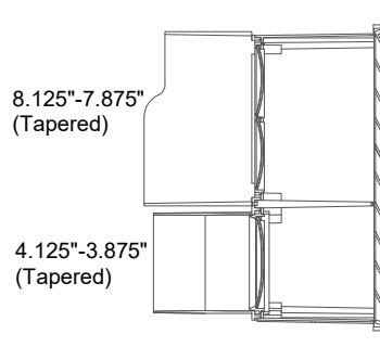
SECTIONAL VIEWS
