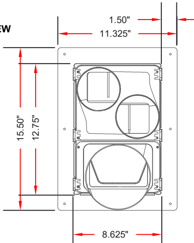
SECTIONAL VIEWS
