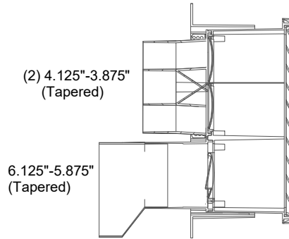
SECTIONAL VIEWS
