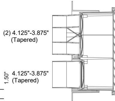
SECTIONAL VIEWS
