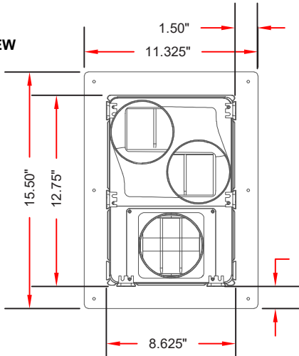
SECTIONAL VIEWS
